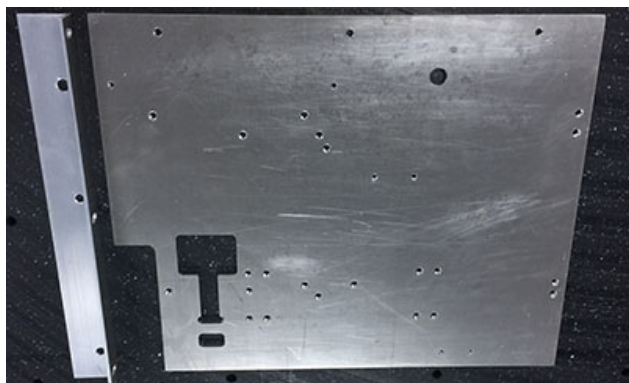
Fig. 13 – Controller plate mounting bracket
