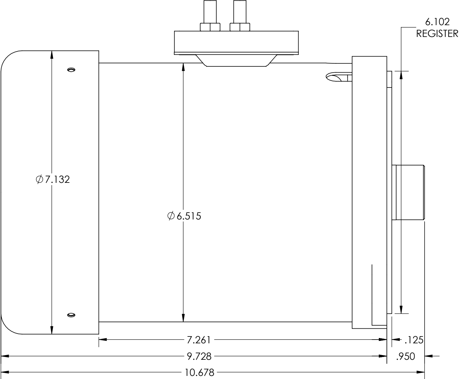
SIDE VIEW
