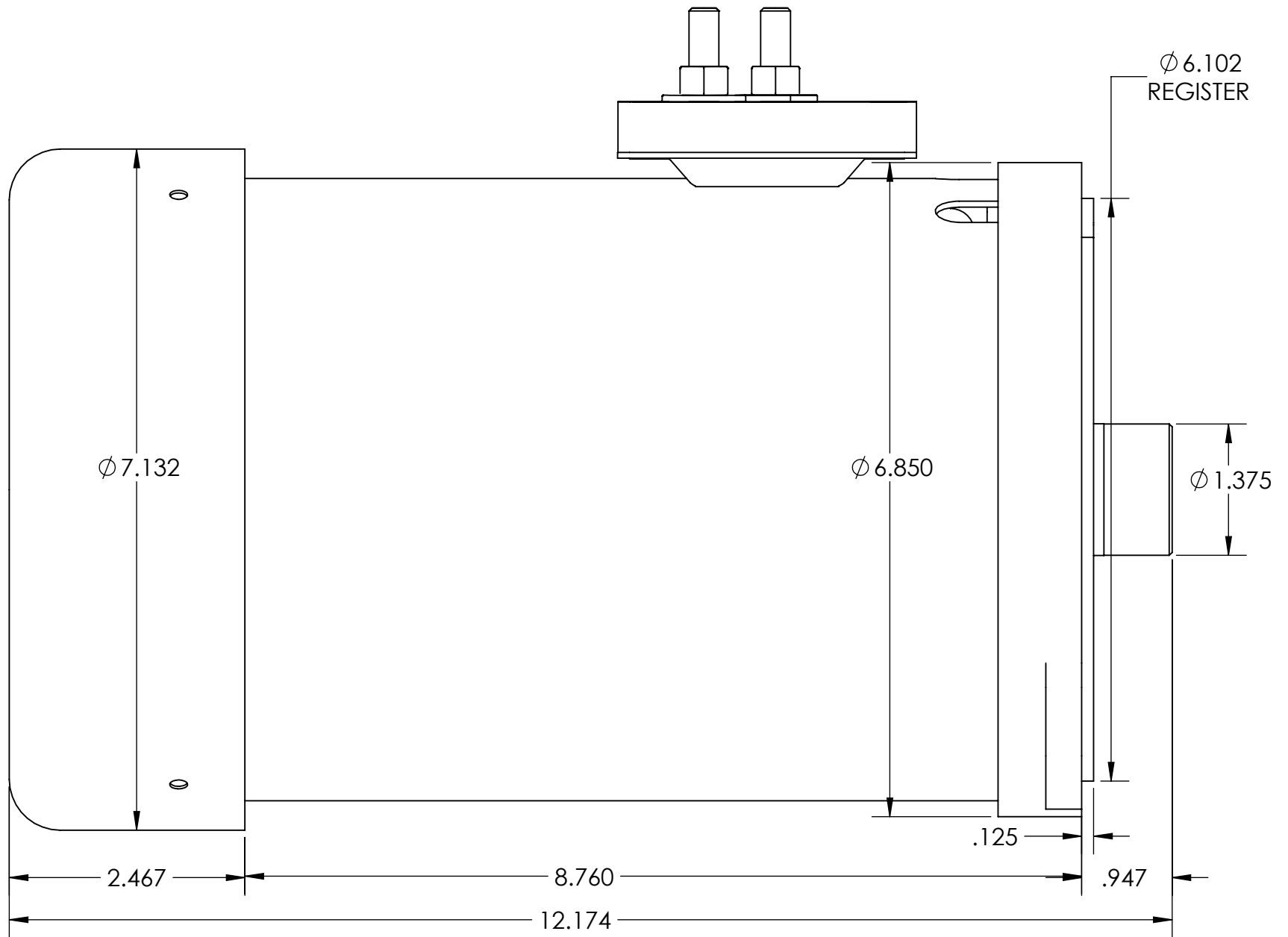
SIDE VIEW
