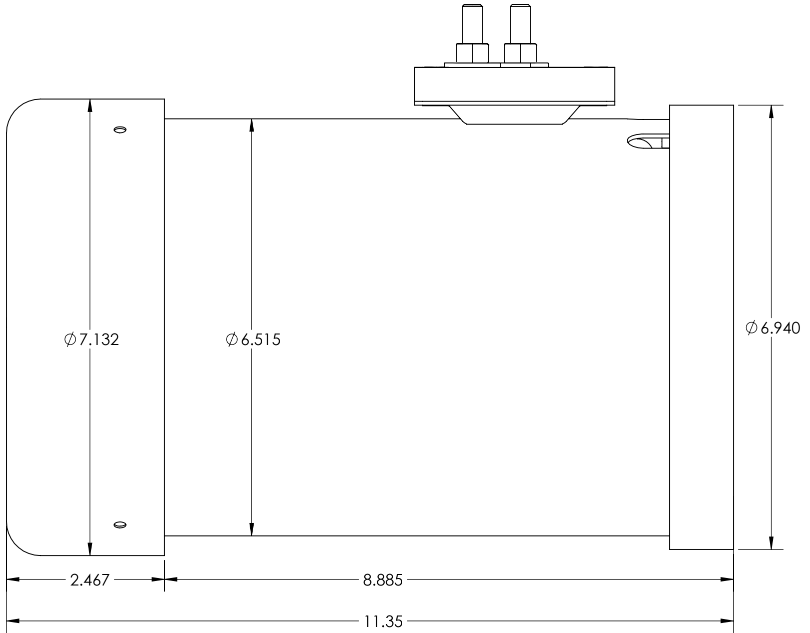
SIDE VIEW
