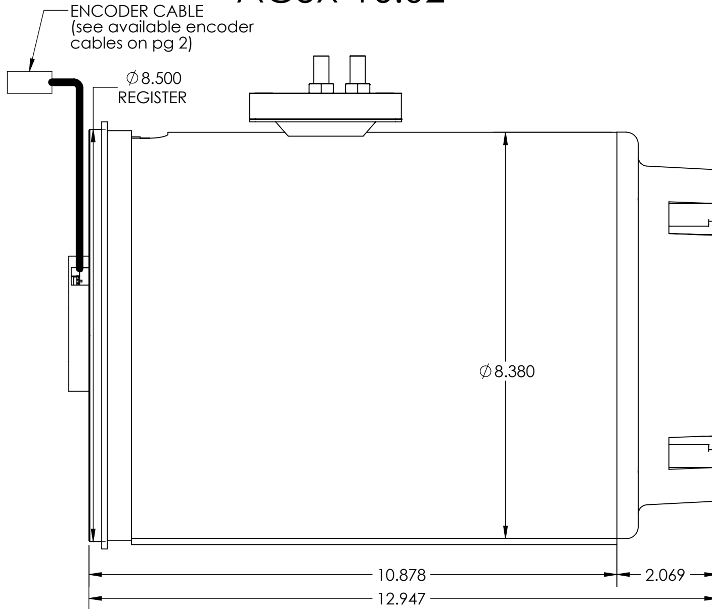
SIDE VIEW
