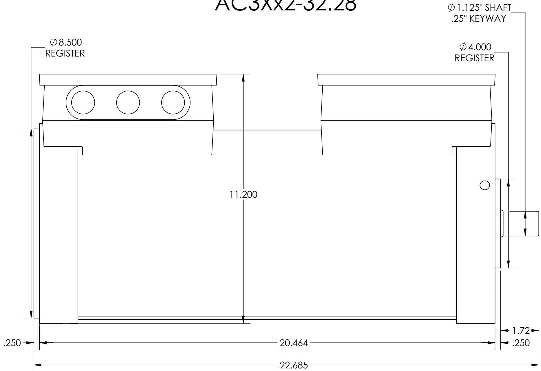
SIDE VIEW
