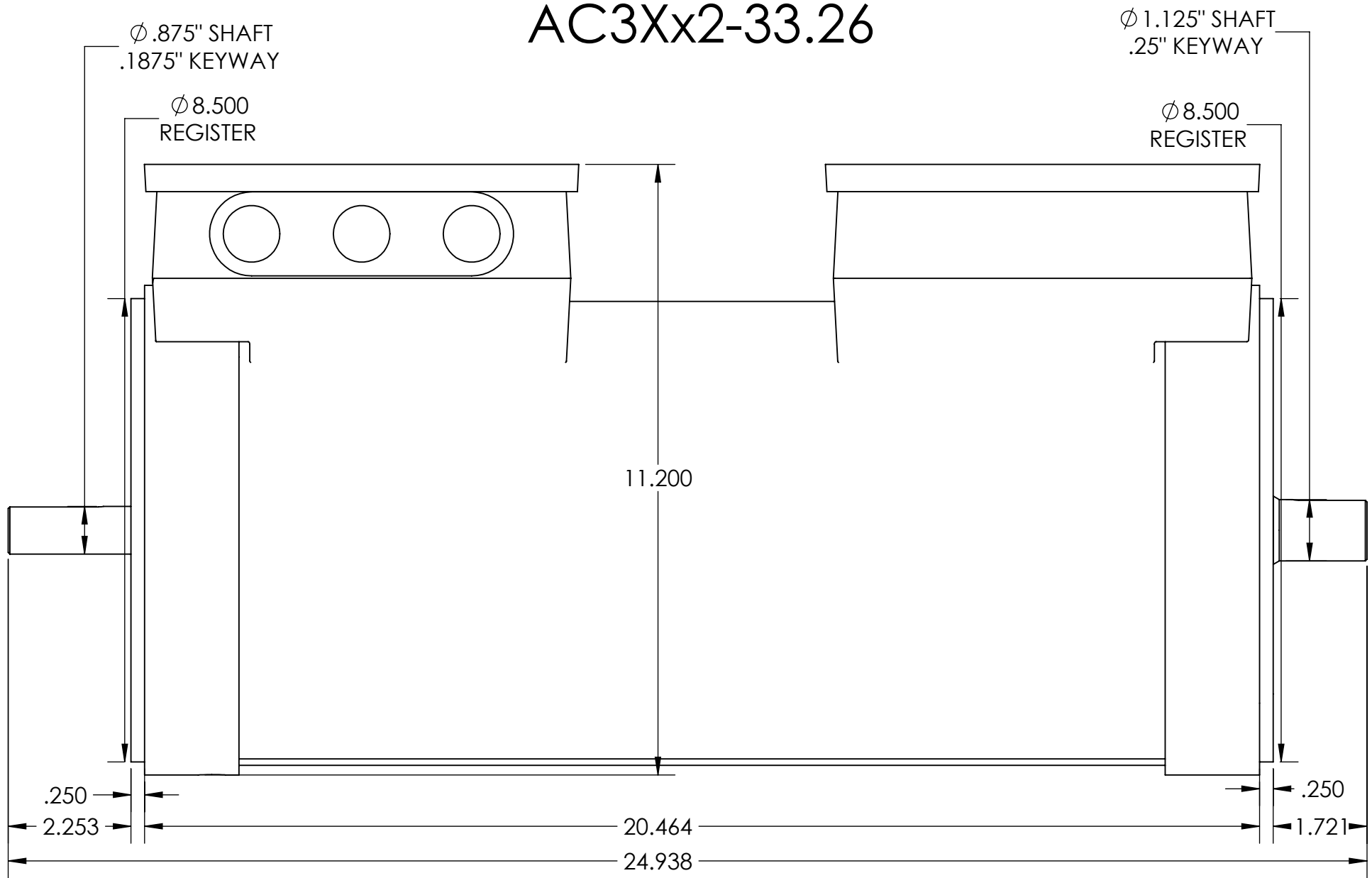
SIDE VIEW
