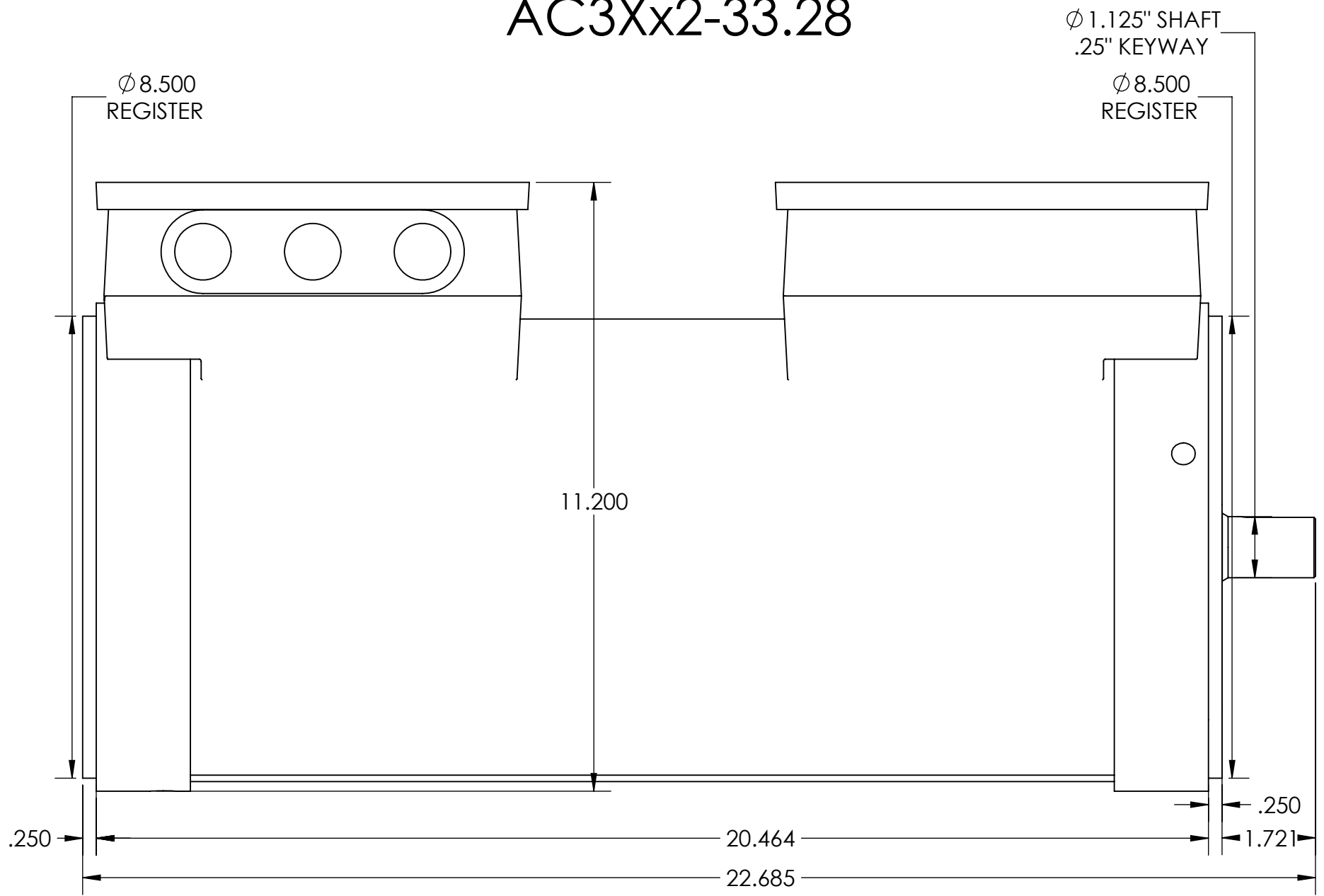
SIDE VIEW
