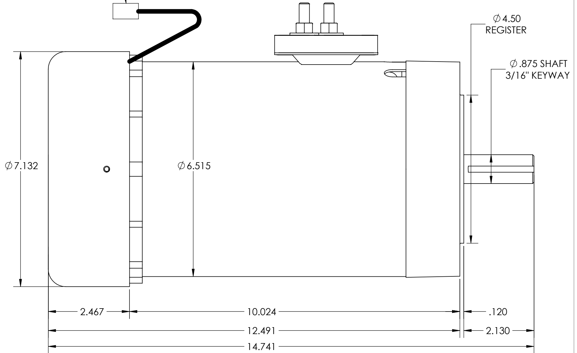
SIDE VIEW
