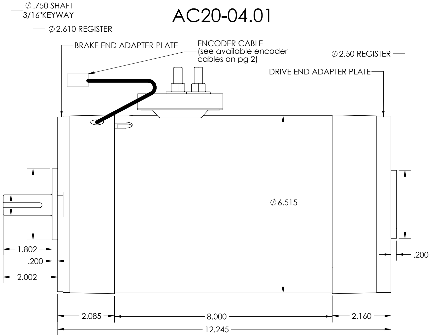
SIDE VIEW
