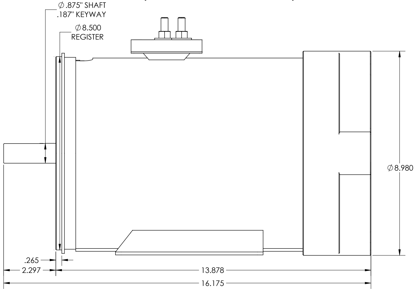
SIDE VIEW
