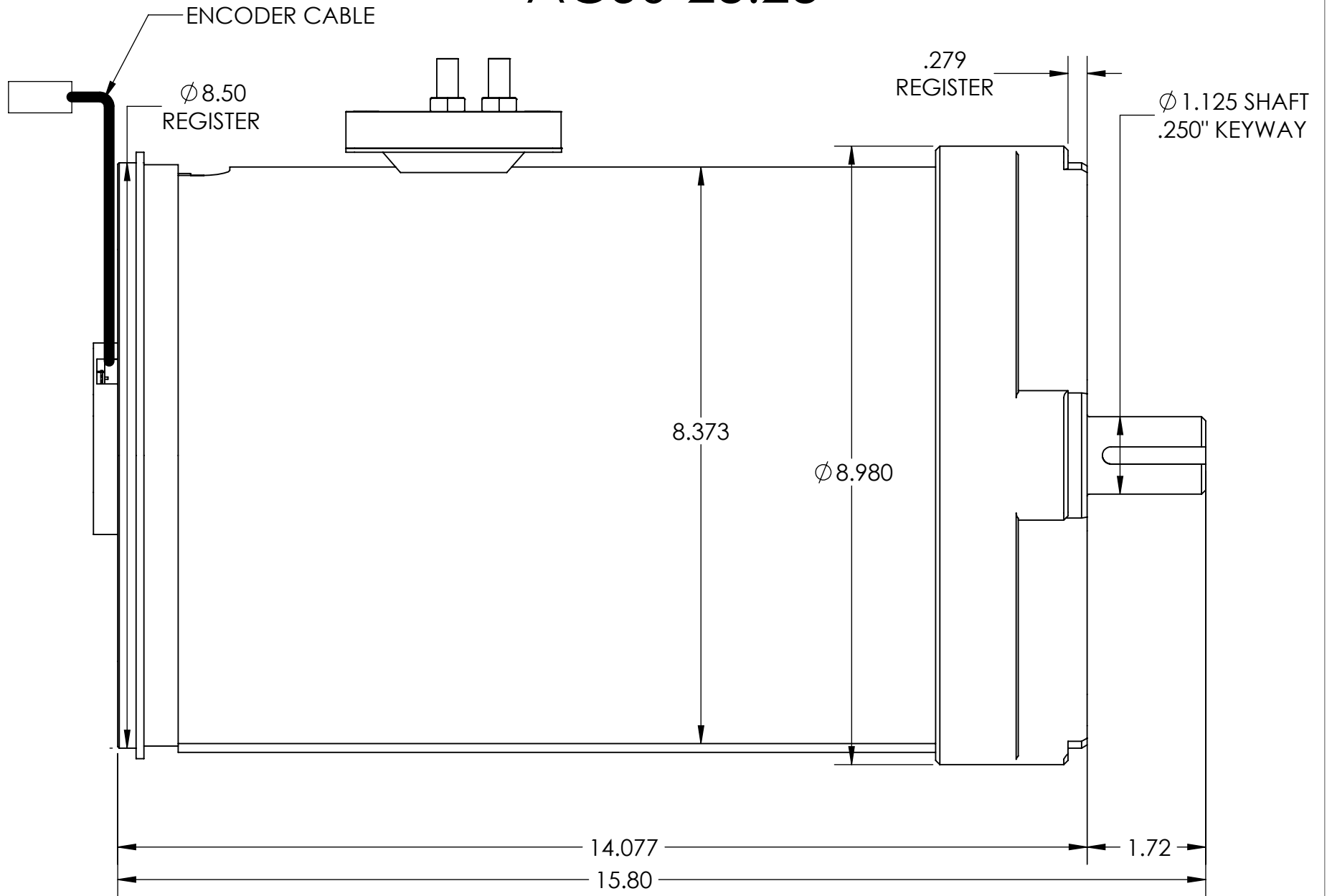
SIDE VIEW
