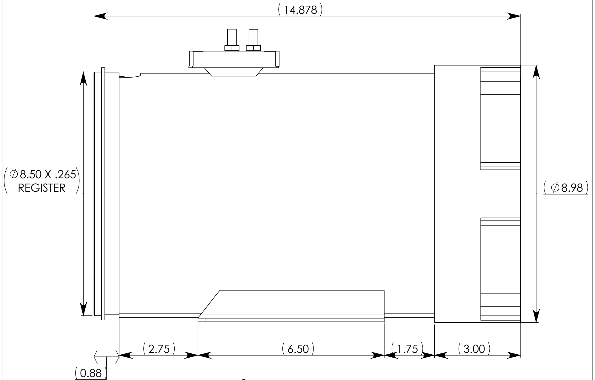
SIDE VIEW
