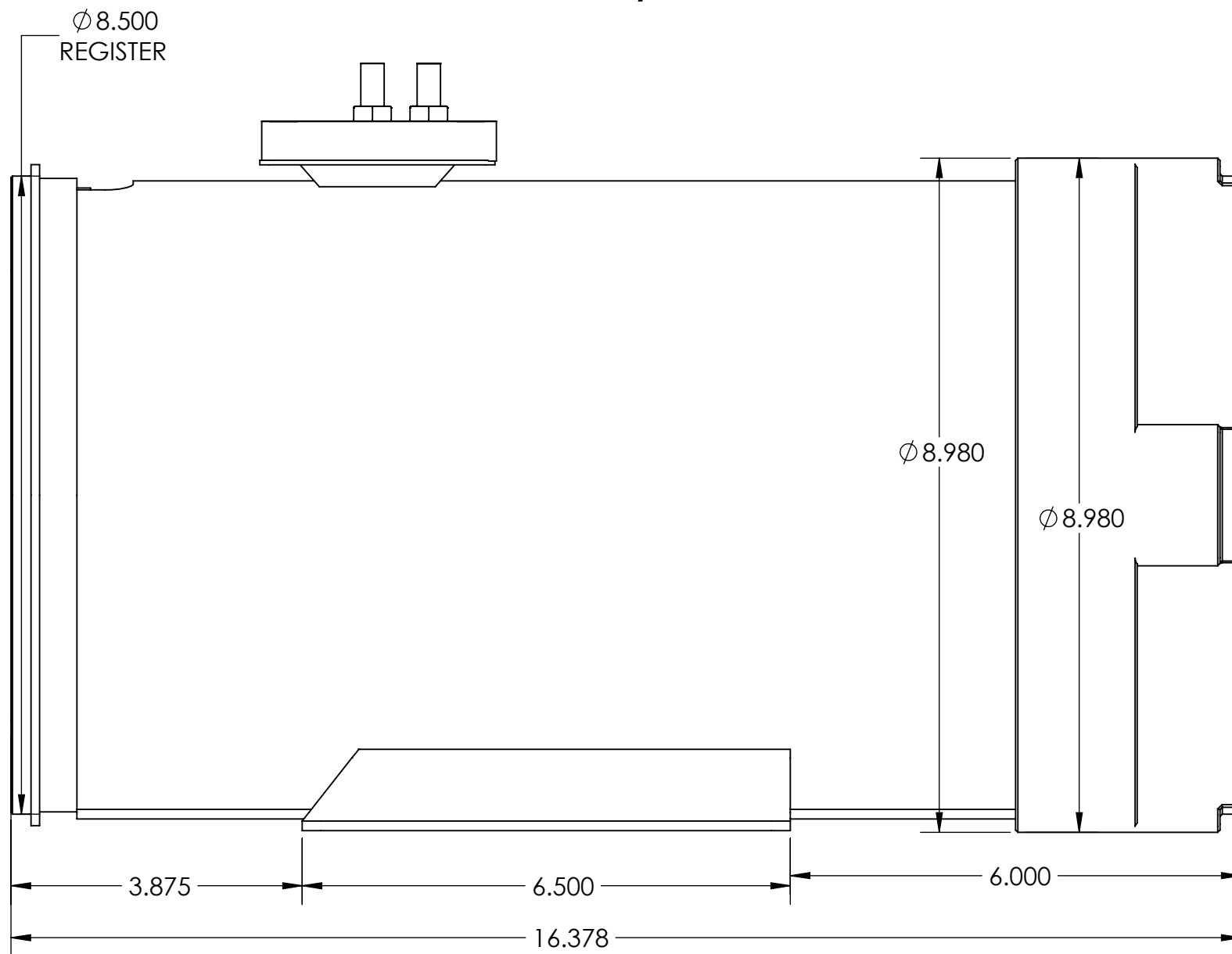
SIDE VIEW
