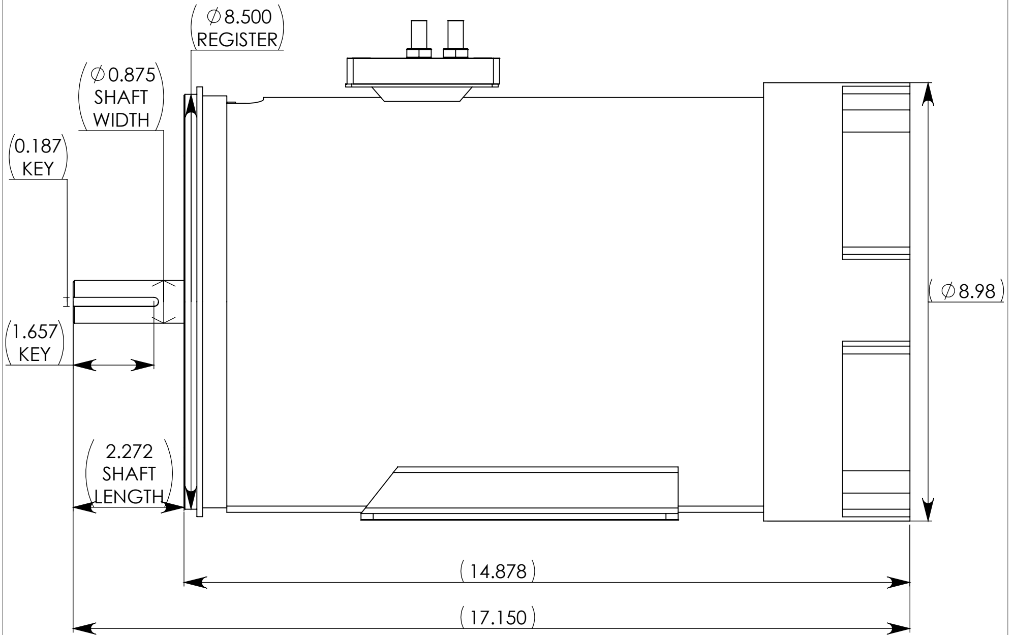
SIDE VIEW
