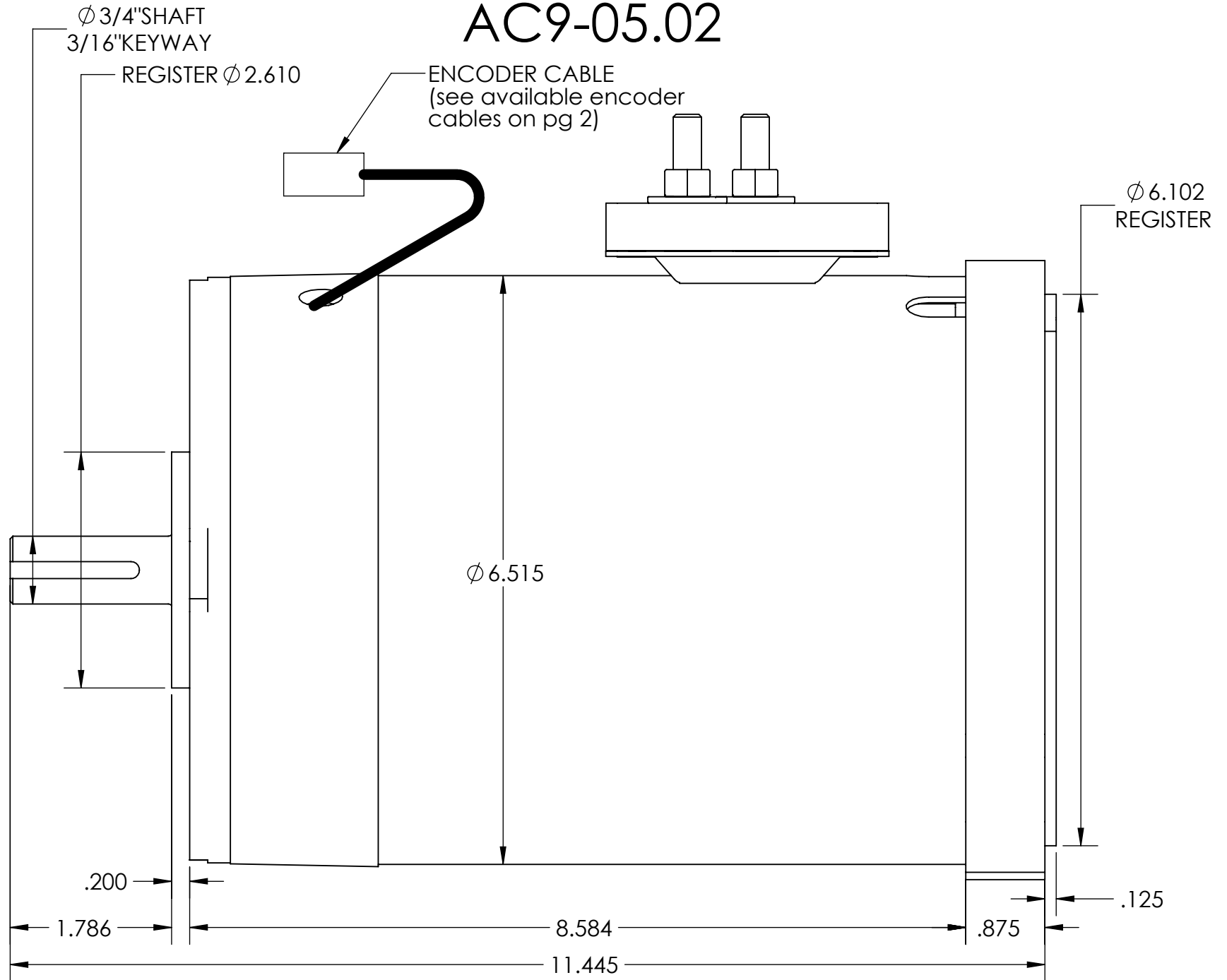
SIDE VIEW
