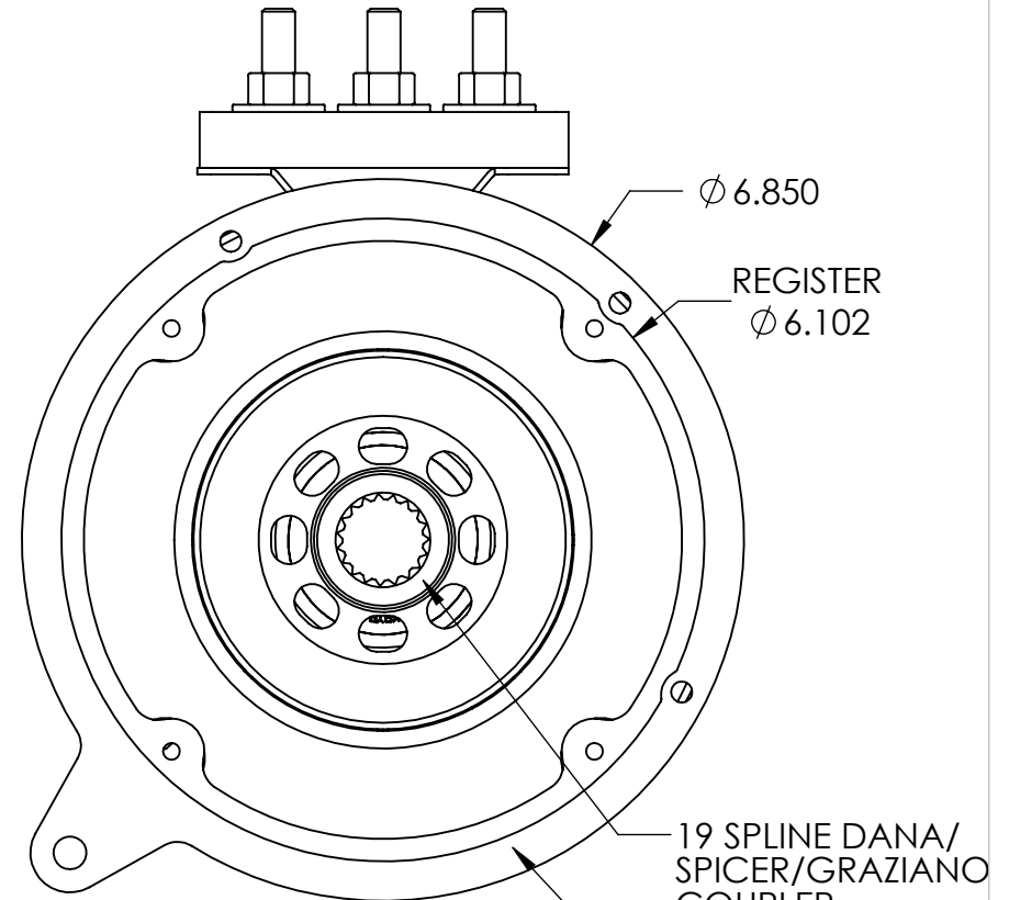
DRIVE END
