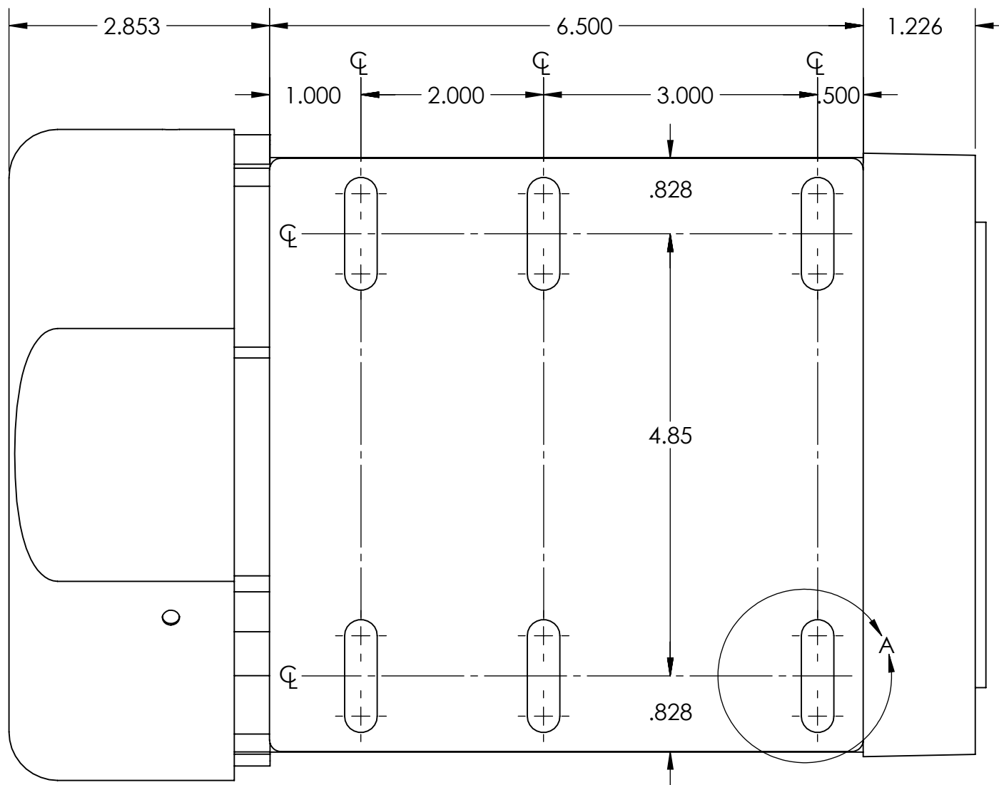
BOTTOM VIEW (MOUNTING LAYOUT)
