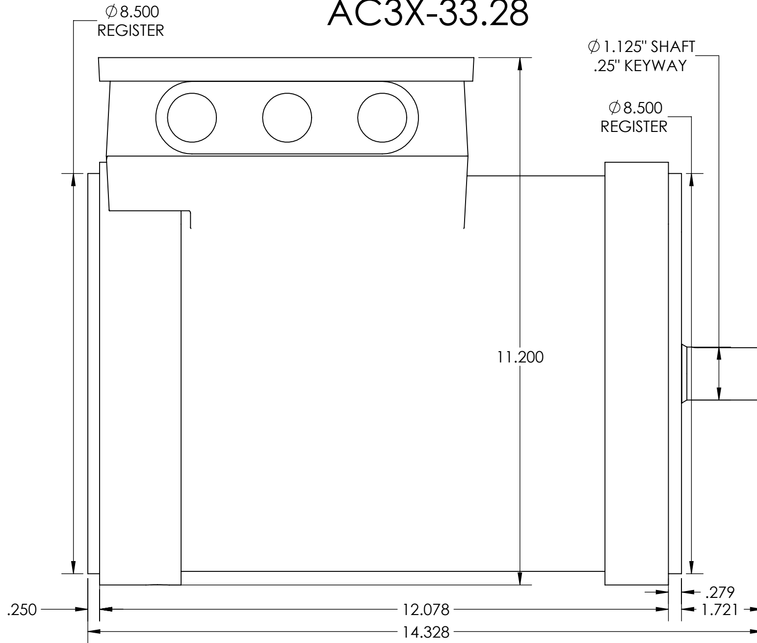
SIDE VIEW
