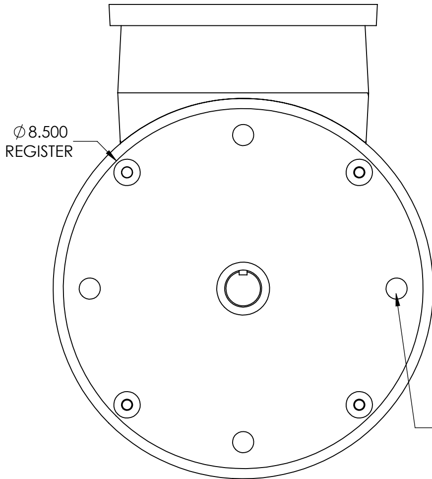
OPPOSITE DRIVE END
