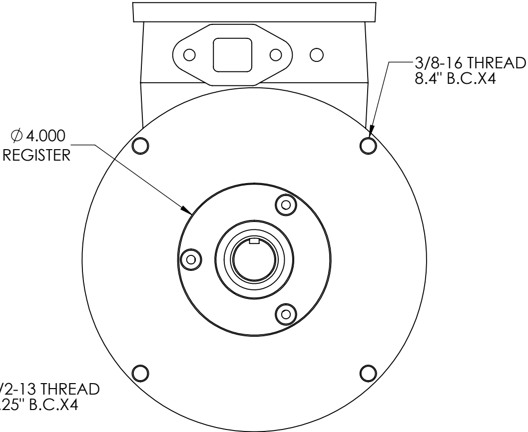
DRIVE END
