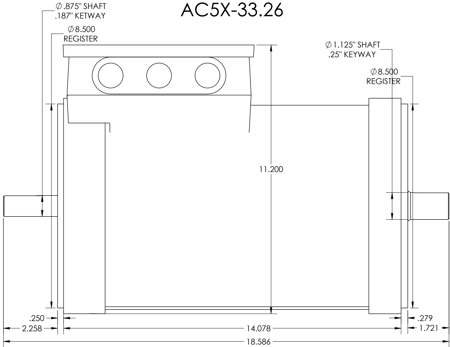
SIDE VIEW
