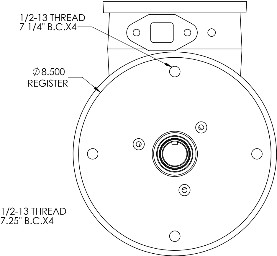
DRIVE END
