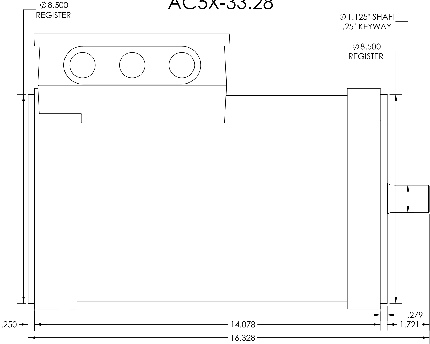
SIDE VIEW
