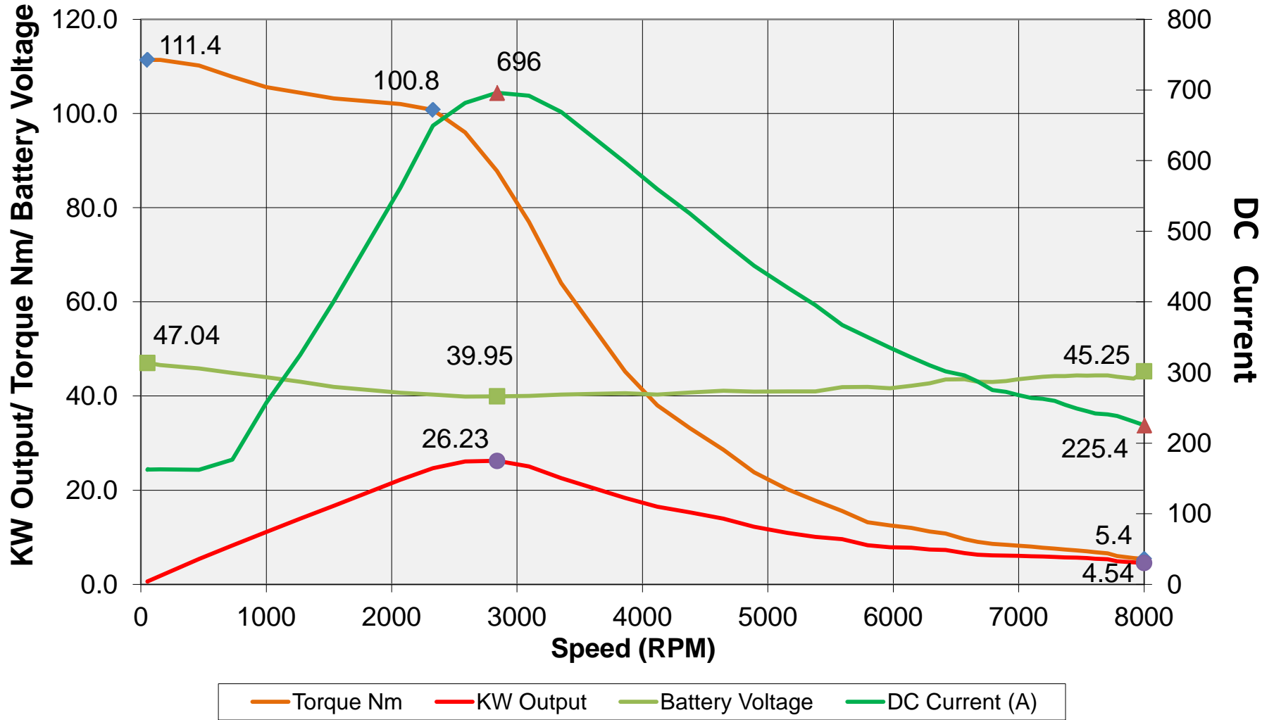
HPEVS AC-20 Metric Peak Graph 48 Volts/650 Amps
