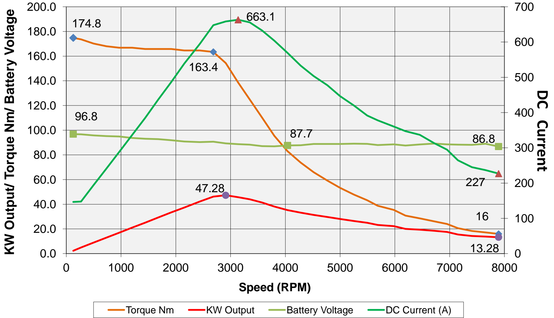
HPEVS AC-35 Metric Peak Graph 96 Volts/650 Amps
