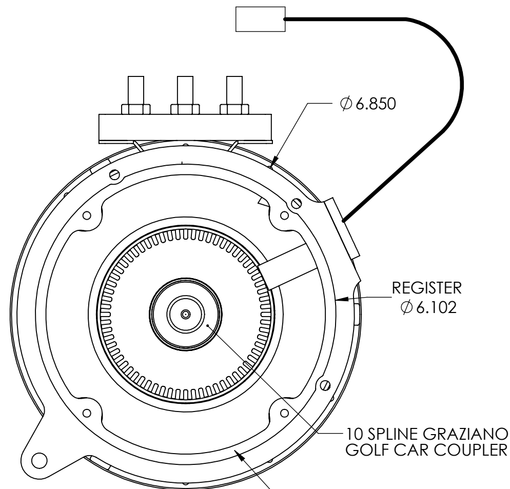
DRIVE END
