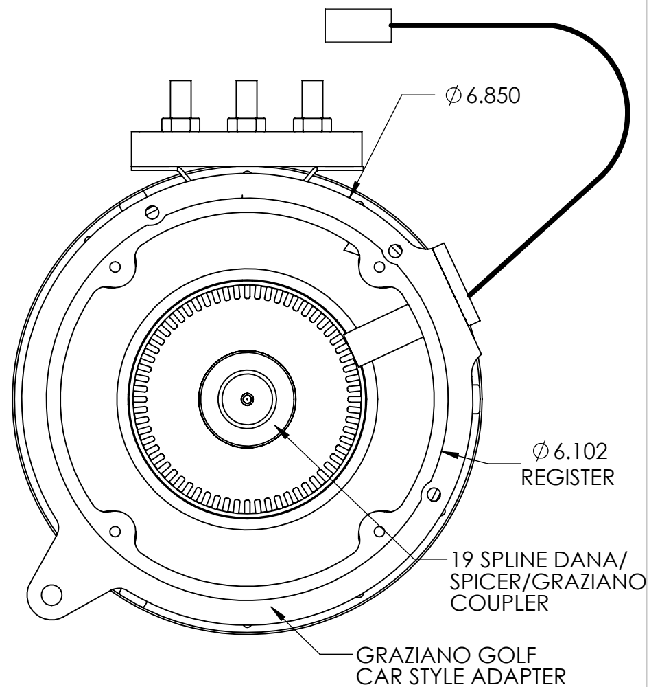
DRIVE END
