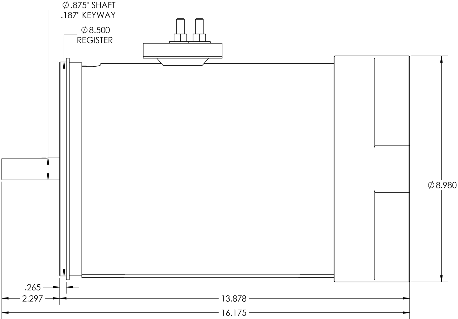
SIDE VIEW
