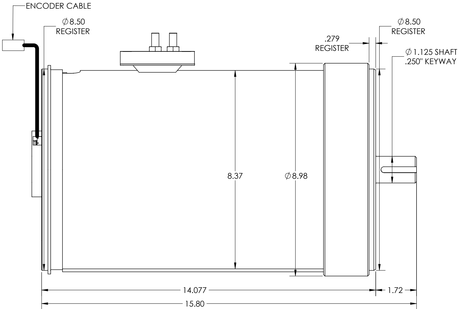
SIDE VIEW
