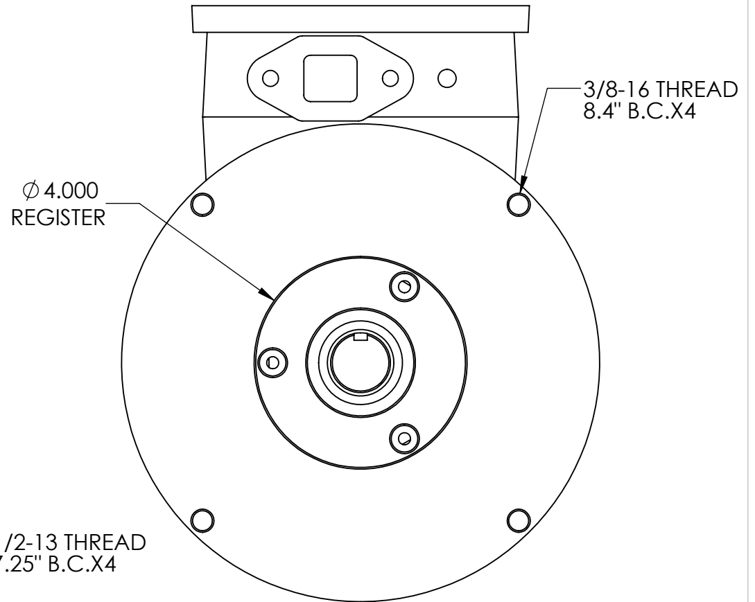
DRIVE END
