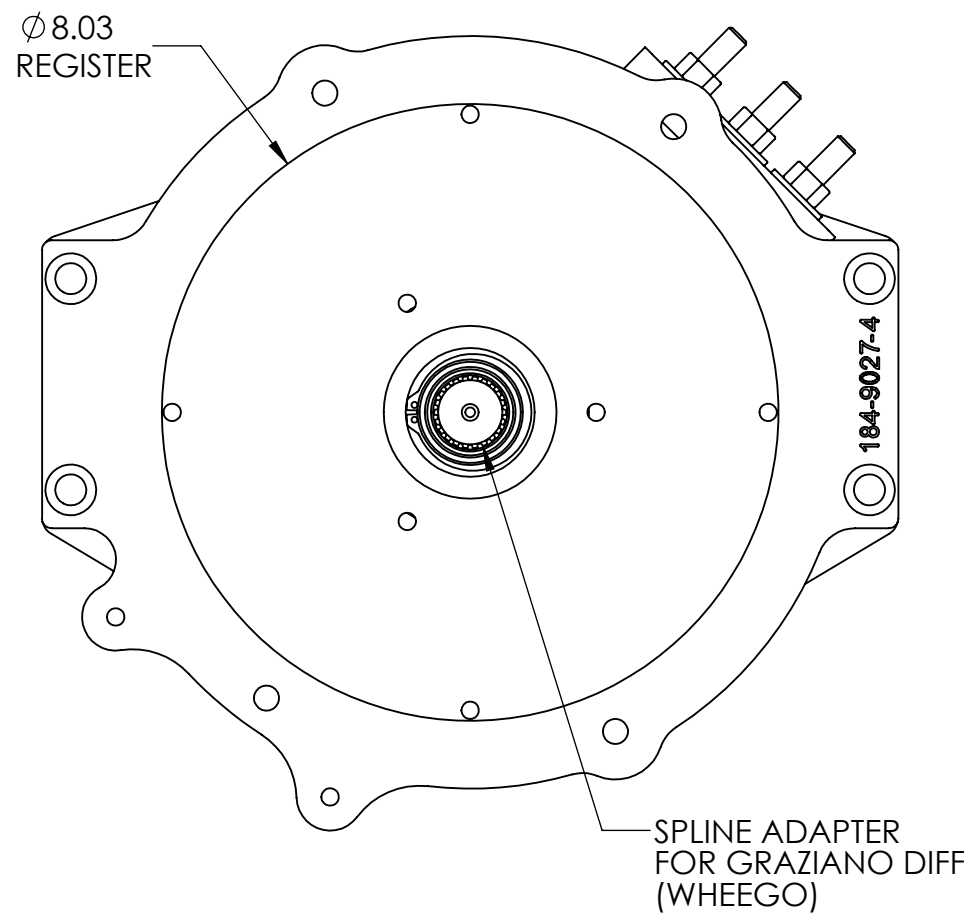
DRIVE END
