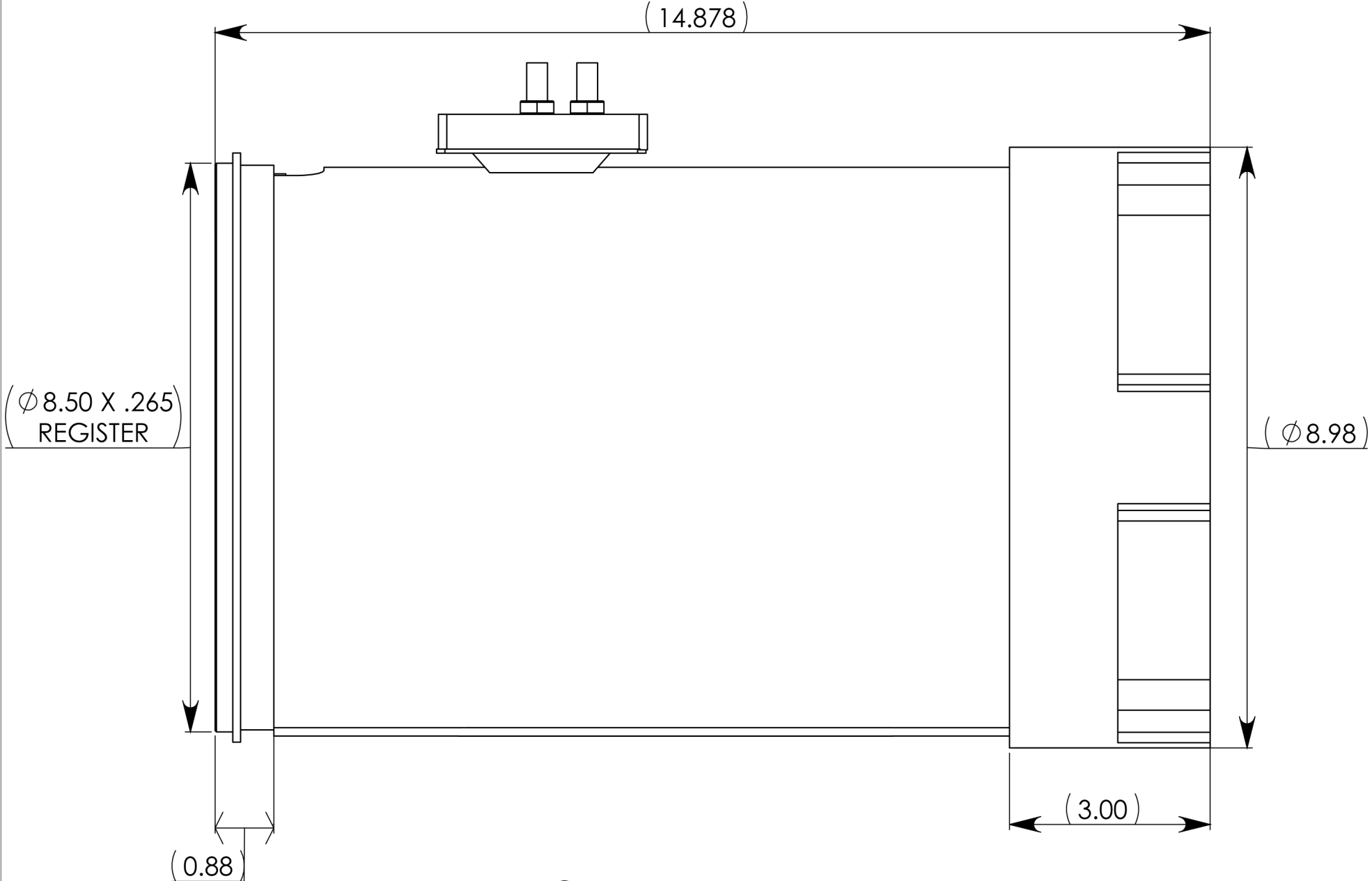
SIDE VIEW
