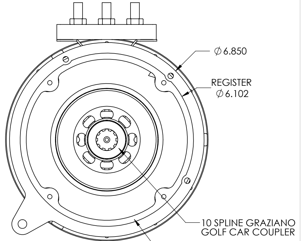
DRIVE END
