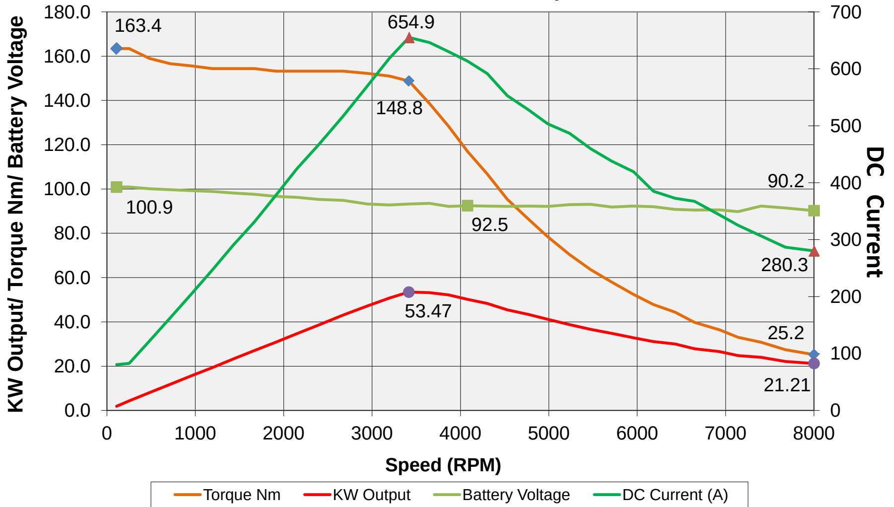
HPEVS AC-50 Metric Peak Graph 96 Volts/650 Amps
